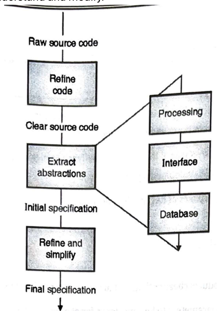
Fig. 10.3.1 : A Reverse Engineering Process
